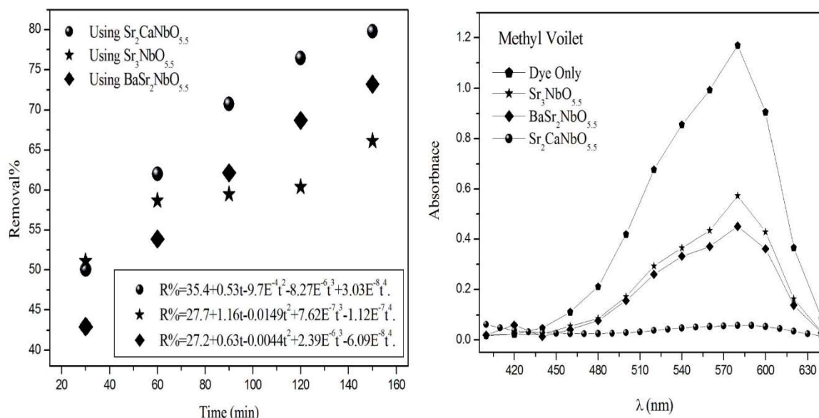
Figure 2. the time dependence of MV removal and The wavelength dependence of absorbance for MV solution at room temperature. The volume, concentration and pH of the dyes solution are 50ml, 10ppm and 5.1 respectively.
